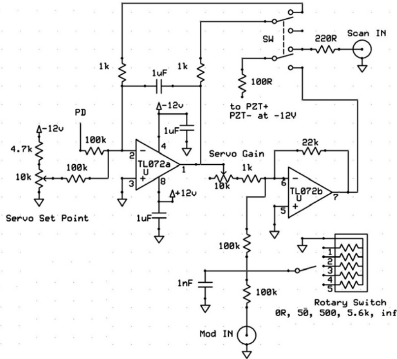
Figure 4. The electronics used to scan, lock, and modulate the interferometer signal. With switch SW in the SCAN position, a signal input to the Scan IN port is sent essentially directly to the PZT. With the switch in the LOCK position, a feedback loop locks the Mirror/PZT so the average photodiode signal (PD) equals the Servo Set Point. With the interferometer locked, a signal sent to the Mod IN port additionally modulates the mirror position. A resistor divider is used to turn off the modulation or reduce it's amplitude by a factor of 1, 10, 100, or 1000.
