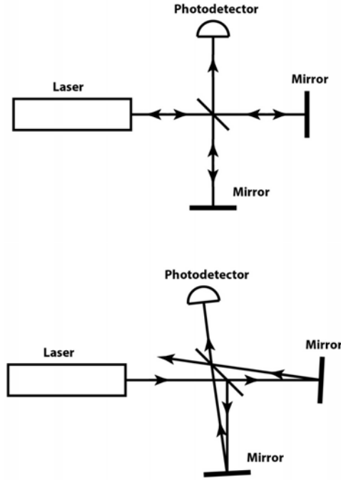
Figure 2. Although the top diagram is often used to depict a basic Michelson interferometer, in reality this configuration is impractical. Reflections from the front mirror of the laser produce multiple interfering interferometers that greatly complicate the signal seen at the photodetector. In contrast, the lower diagram shows how a slight misalignment (exaggerated in the diagram) eliminates these unwanted reflections without the need for additional optical elements. In the misaligned case, however, complete overlap of the recombined beams is only possible if the arm lengths of the interferometer are equal.
