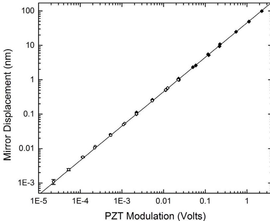
Figure 7. The measured mirror displacement when the piezoelectric transducer was driven with a square wave modulation at 600 Hz, as a function of the modulation amplitude. The high-amplitude points (closed diamonds) were measured by observing the photodiode signal directly on the oscilloscope, while the low-amplitude points (open circles) were measured using the phase-sensitive averaging circuit shown in Figure 6. The fit line gives a PZT response of 45 nm/volt. These data indicate that the combined PZT and photodiode responses are quite linear over a range of five orders of magnitude in amplitude. At the lowest modulation amplitudes, the noise in the averaged interferometer signal was below one picometer for 10-second averaging times.
