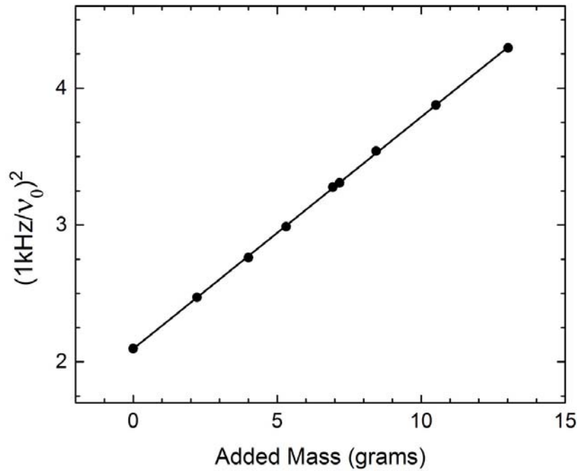
Figure 11. Measured changes in the resonant frequency \nu_0 of the oscillator as a function of the mass added to the mounting hole shown in Figure 9. Simple-harmonic-oscillator theory predicts that \nu_0^{-2} should scale linearly with added mass. The spring constant and moment of inertia of the oscillator can be extracted from the slope and intercept of the fit line.
