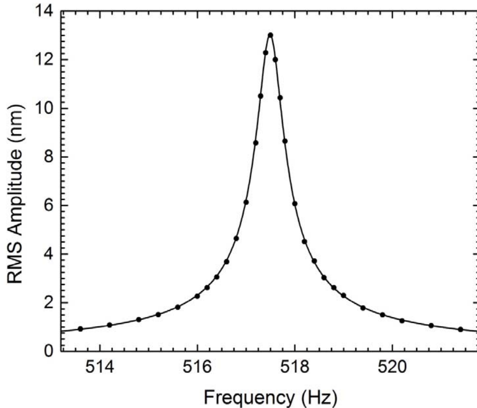
Figure 10. The measured resonant response of the oscillator as a function of drive frequency. The absolute root-mean-square (RMS) amplitude was derived optically from the interferometer signal. The response is well matched by a simple-harmonic-oscillator model (fit line), indicating a mechanical Q of 970.
