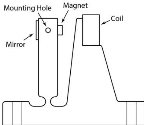
Figure 9. A side view of the magnetically driven mechanical oscillator shown in Figure 8. The main body is constructed from 12.7-mm-thick aluminum plate (alloy 6063), and the two vertical holes in the base are 76.2 mm apart to match the holes in the breadboard. Sending an alternating current through the coil applies a corresponding force to the permanent magnet, driving torsional oscillations of the mirror arm about its narrow pivot point. Additional weights can be added to the 8-32 tapped mounting hole to change the resonant frequency of the oscillator.
