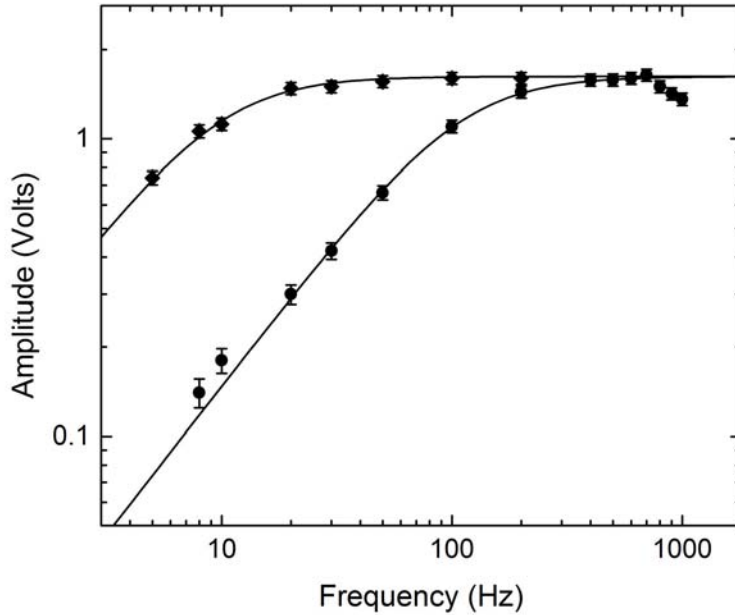
Figure 5. Measurements of the interferometer response as a function of the PZT modulation frequency, with the servo locked. The upper and lower data points were obtained with the servo gain at its lowest and highest settings, respectively, using the servo control circuit shown in Figure 4. The theory curves were derived from an analysis of the servo control circuit, using parameters that were measured or derived from circuit elements. To better match the data, the two theory curves each include an additional multiplicative factor of 0.94, consistent with the estimated overall uncertainty in determining the circuit parameters.
