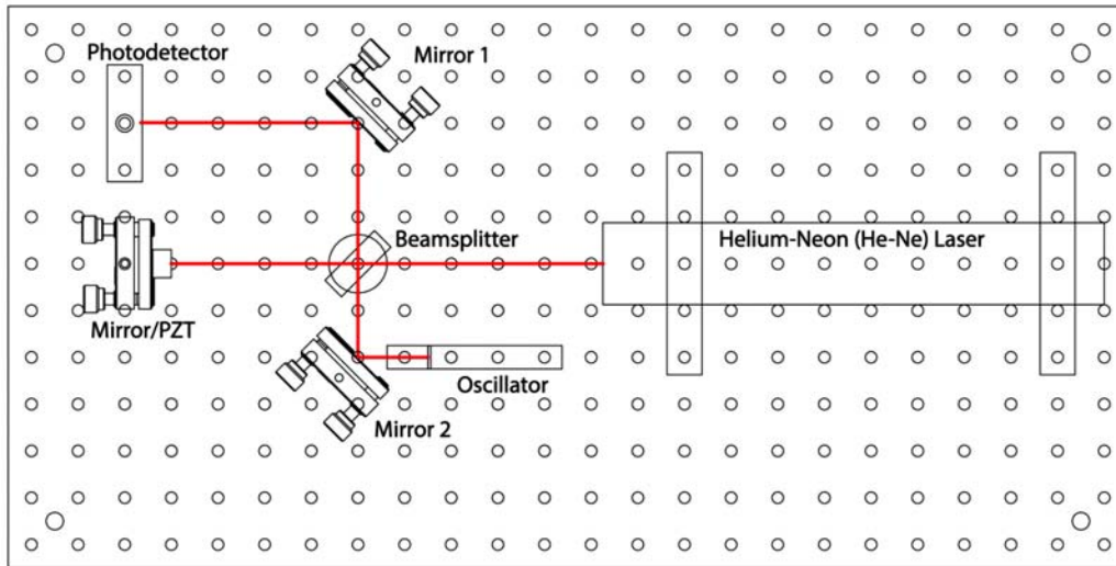
Figure 8. The interferometer optical layout including the mechanical oscillator shown in detail in Figure 9.
