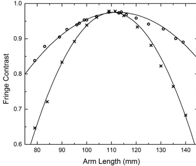
Figure 3. The measured fringe contrast F_{C,\max} as a function of the length of the Mirror 2 arm of the interferometer. For each data point, Mirror 2 was repositioned and reclamped, and then the Mirror 2 pointing was adjusted to obtain the maximum possible fringe contrast. The “X” points were taken with a Mirror/PZT misalignment of 4.3 mrad (relative to retroreflection), while the circles were taken with a misalignment of 1.3 mrad. The lines show parabolic fits to the data.
