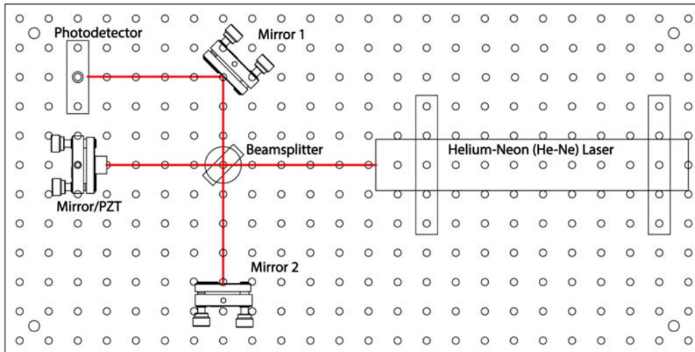
Figure 1. The interferometer optical layout on an aluminum breadboard with mounting holes on a 25.4-mm grid. The Mirror/PZT consists of a small mirror glued to a piezoelectric stack mounted to a standard optical mirror mount. Mirrors 1 and 2 are basic steering mirrors, and the Beamsplitter is a wedge with a 50:50 dielectric coating.
